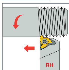
Right-Hand Thread
