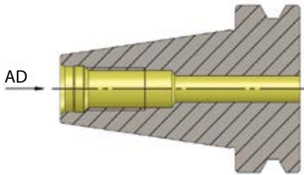
Form AD Through Spindle Coolant
