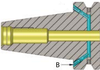
Form AD/B Through Spindle Coolant & Through Flange Coolant
